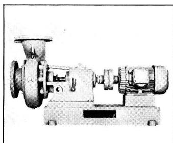
Pompes basse-pression
