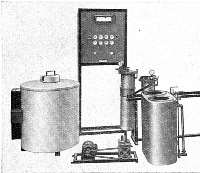
Installation de recuit blanc-brillant
