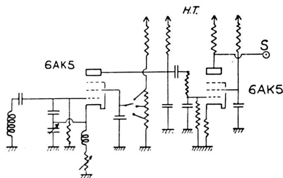
Montage autodyne + 1 lampe BF
