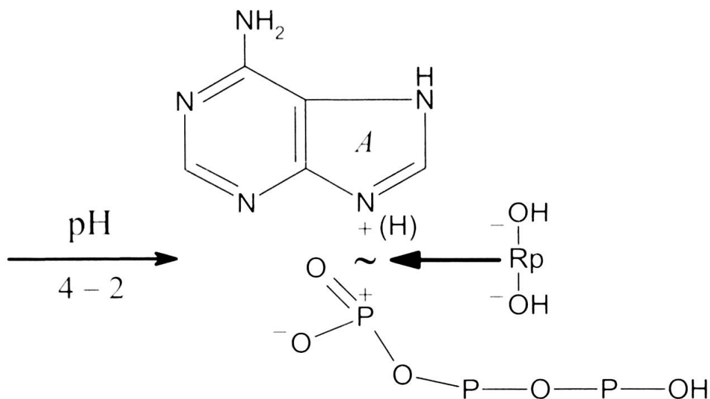
FIG. 1. Final step in the prebiotic origin of adenosine triphosphate implies acid-opening (pH < 4) P~N of the bonding between adenine (A) and triphosphate and further bridging by amphihydroxylated ribose precursors (Rp). For the initial steps of P~N bonding on “low tautomerized” adenine, see Fig.1 in TURIAN (2001a,b).
