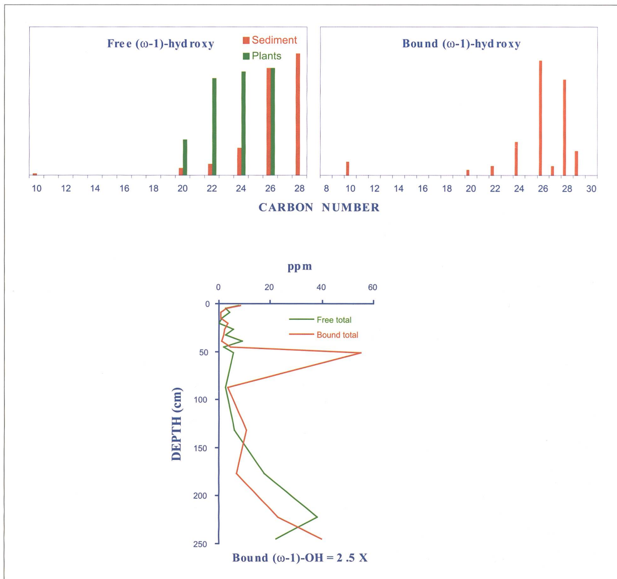
Fig. 8. Histograms of ( \omega -1)-hydroxyacids normalized to C_{26,0} in the free and bound fractions of lake Cadagno surface sediments and plants (top). Depth profiles of free and bound total ( \omega -1)-hydroxyacids (bottom). Abundances in ppm should be multiplied by indicated factors for species given under the graphs.
