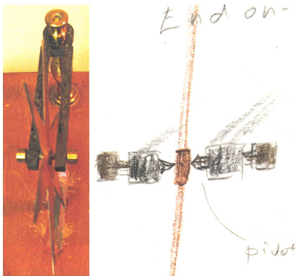
Fig. 8. Edge-on photo and my sketch of mounting of Barlow star wheel between pointed screw tips (Bakken Museum 96.5.3).
