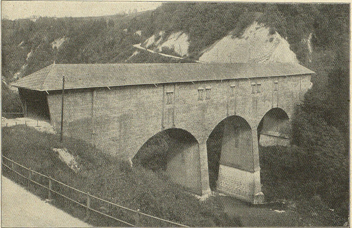
Gundwilertobel-Brücke.
