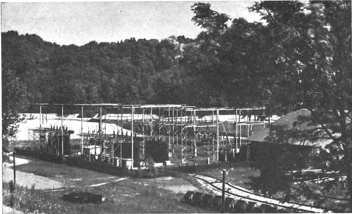
Fig. 26. 150 kV-Freiluft-Transformatorstation.
