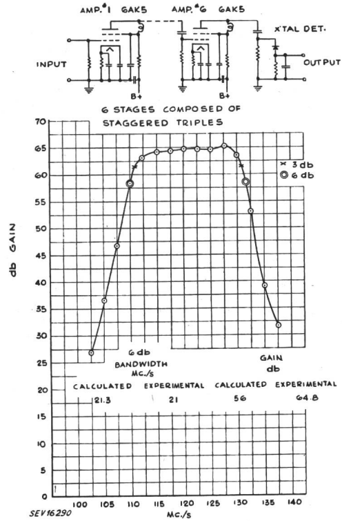
Fig. 10 Frequency Response of 120 Mc./s IF Amplifier
