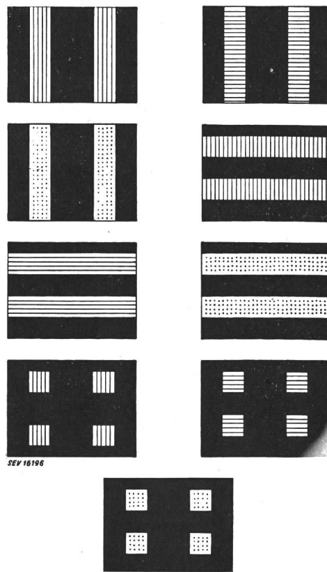
Fig. 3 Artificial Patterns
