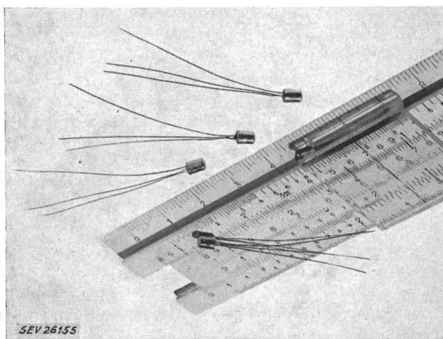
Fig. 1 Philips-Transistor OC 57
