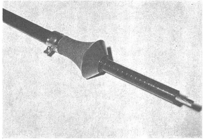
Fig. 15 Stress-Cone 20 kV
