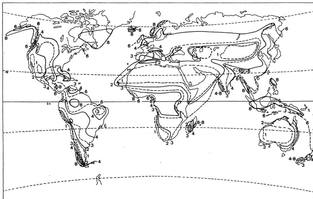
Fig. 4. Aridity factor of Martonne i: Coefficient of the mean annual rainfall in cm divided by the mean annual temperature in ^{\circ}\text{C} + 10 .
