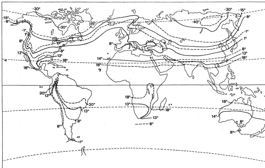
Fig. 3. Mean winter temperatures (three coolest months)
