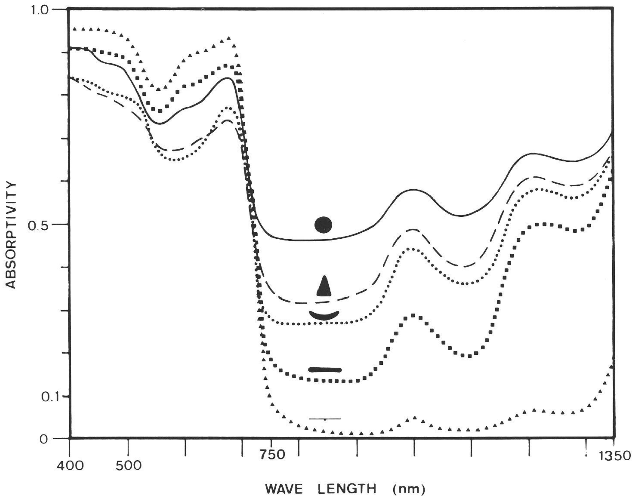
Fig. 3 Absorptivities of leaves with different leaf expansion coefficients S (surface in \text{cm}^2 /fresh weight in g). Inserted into the fig. are sketches of leaf crosssections. ——— Othonna opima ( S = 3.91 ), - - - - Cheiridopsis sp. ( S = 3.80 ), ······ Aloe ramosissima ( S = 5.55 ), ■ ■ ■ ■ Tylecodon paniculatus ( S = 8.55 ), ▲ ▲ ▲ ▲ Ozoroa dispar ( S = 41.67 ).
