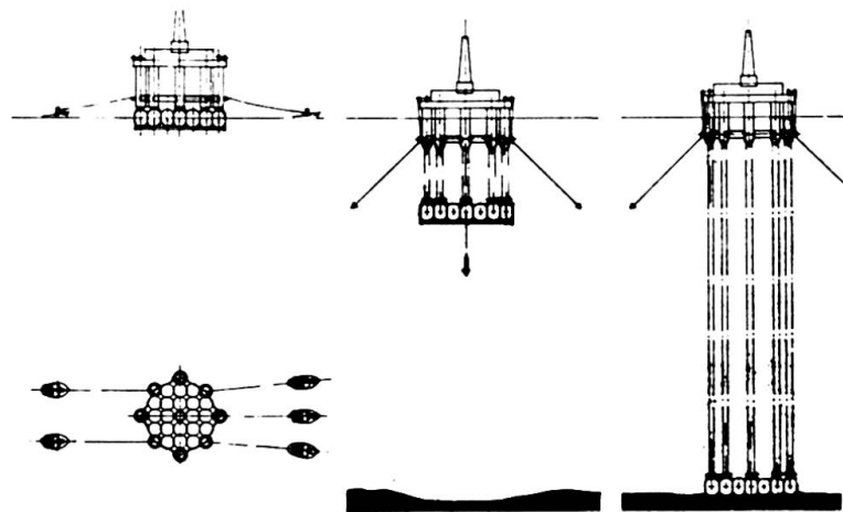
Fig. 24 Diagram of platform installation on the site.
