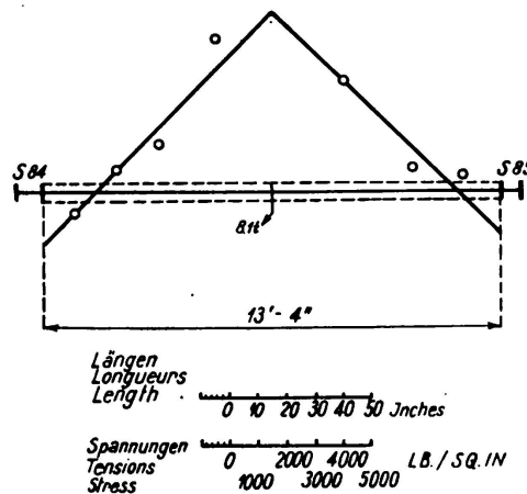
Fig. 4. Observed stress due to torsion when a central concentrated load of 8.1 tons was applied to Beam No. 840 D.
