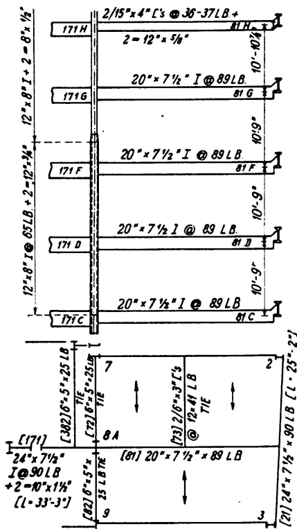
Fig. 3. Unsymmetrical frame of Hotel Building.
