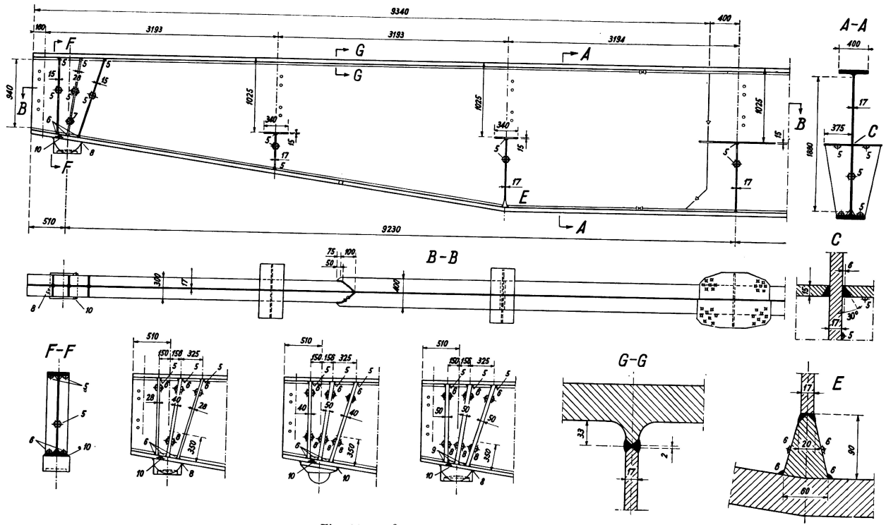
Fig. 11. Pålund Bridge. Cross beams.
