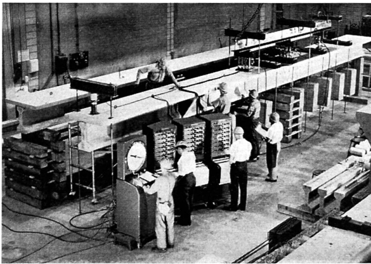
Fig. 9. Shear Test of Composite Prestressed Girder.
