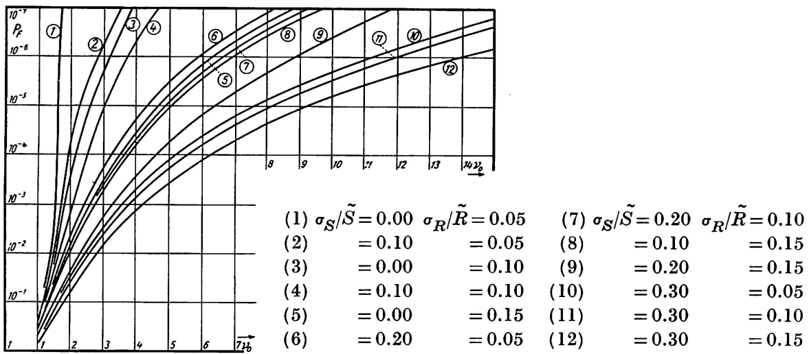
Fig. 1 Relation of "central" safety factor \nu_0 = \tilde{R}/\tilde{S} and probability of failure P_F . (extremal distributions).
