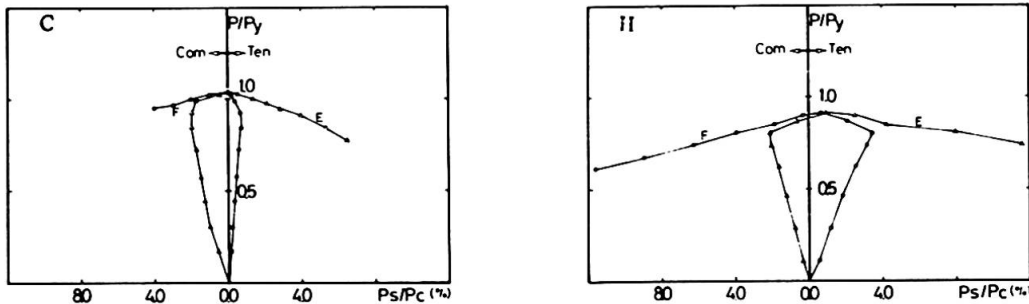
Fig. 10 P/Py-Ps/Pc relationships
