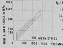
SMITH DIAGRAM AT 2 \cdot 10^6 CYCLES
