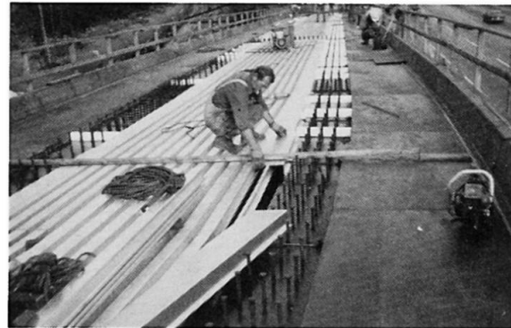
Figure 12. Metal decking.
