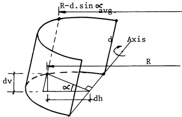
For Plate cutting dv becomes \frac{dv - dh \cdot \tan \alpha}{\cos \alpha}
