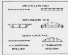
FIG 2 COMPUTATION ILLUSTRATION OF ATC6 SEISMIC DESIGN FORCE
