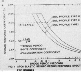
FIG 1 ATC6 ELASTIC SEISMIC DESIGN RESPONSE SPECTRA FOR BRIDGES
