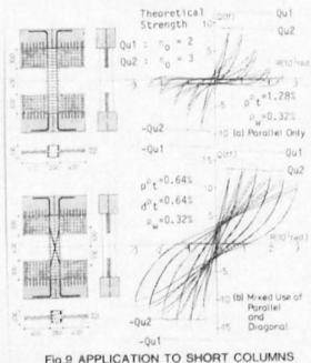
Fig. 9 APPLICATION TO SHORT COLUMNS
