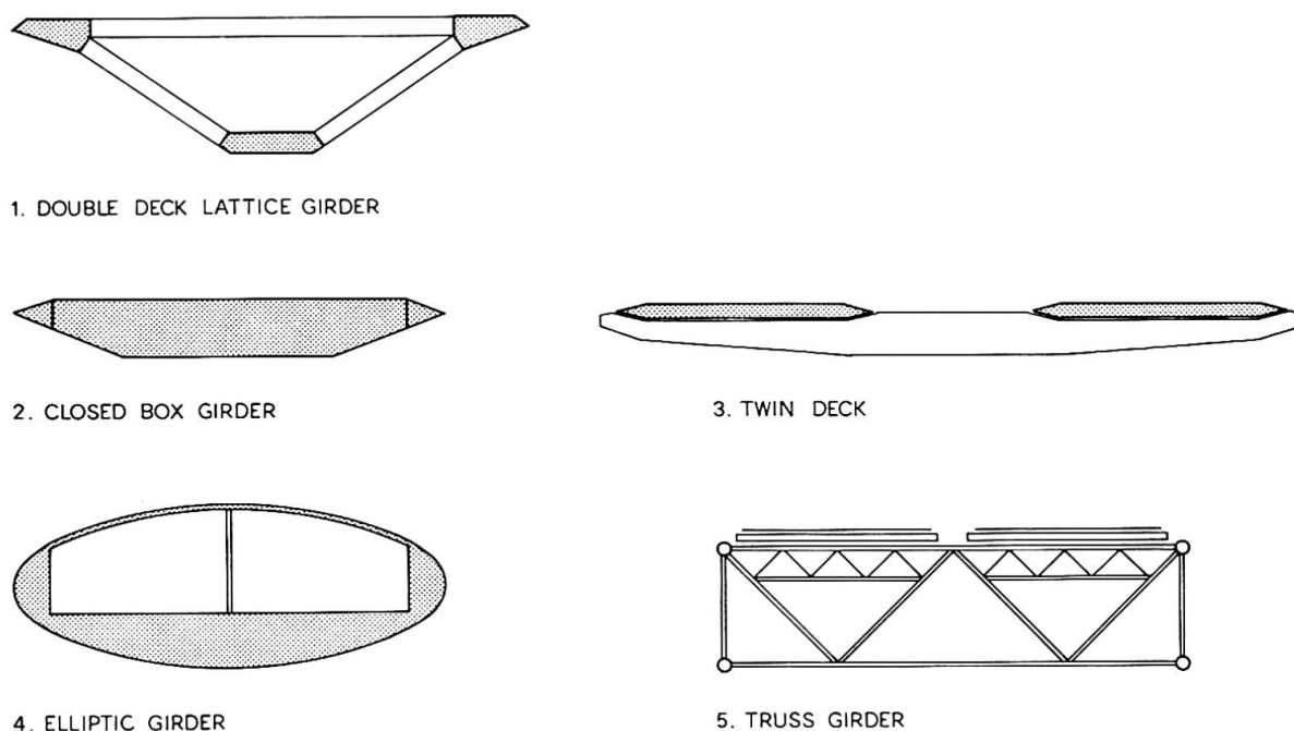
Fig. 3 Girder designs
