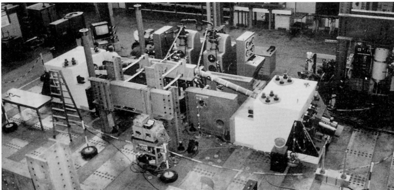
Fig. 3 : VSL stay cable testing at EMPA in Dübendorf, Switzerland
