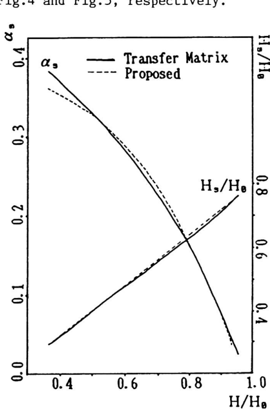
Fig. 3 \alpha_s - H/H_0, H_s/H_0 - H/H_0 relationships
