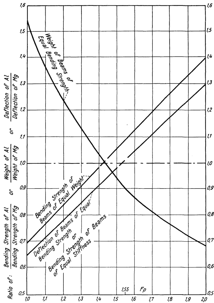
Fig. 1. Comparison of Al and Mg Cantilever Beams of \bar{I} , \bar{I} and Tubes
