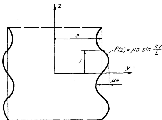
Fig. 4. The shell with surface corrugations.
