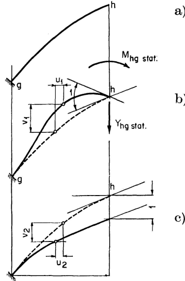
Fig. 3. Static deflection of curved bar.
