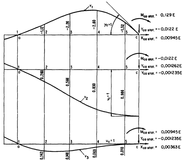
Fig. 6. Deflection curves for unit end-deformations of member "a - c" (vertical ordinates).
