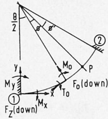
Fig. 17. Point load on a curved girder.
