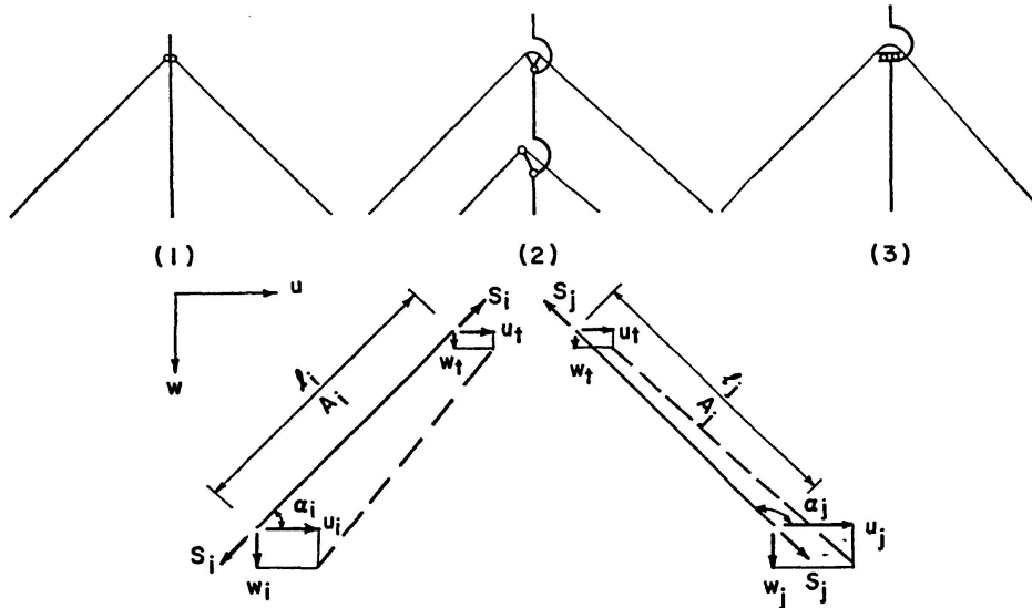
Fig. 2. Cable saddle types and cable forces and displacements.
