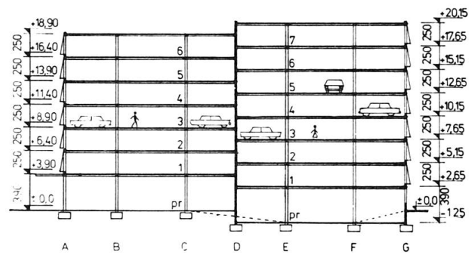
Fig. 3 Typical vertical section
