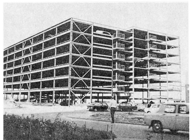
Fig. 4 Steel structures during erection
