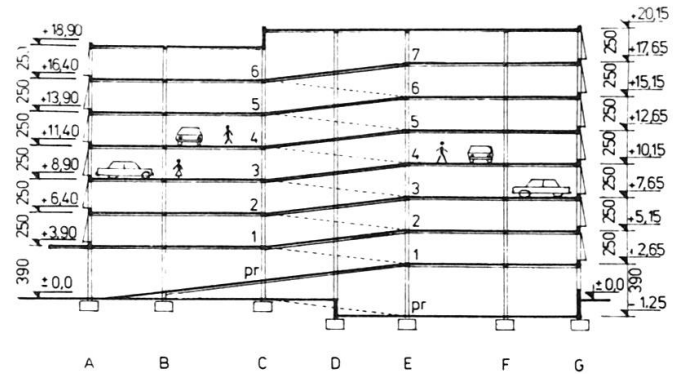
Fig. 2 Vertical section with the ramps
