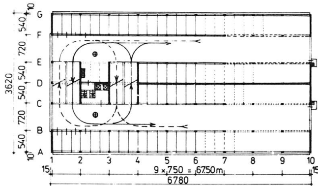
Fig. 1 Typical parking floor
