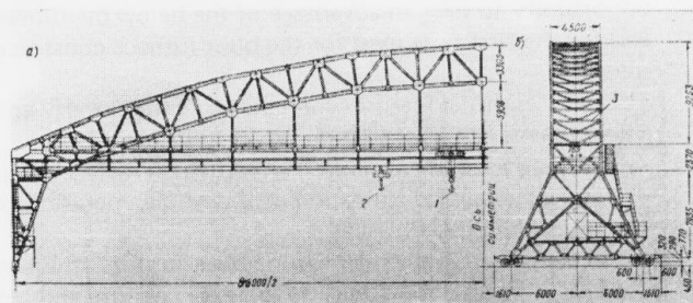
Fig. 2 Gantry Crane Made of Aluminium Alloys
