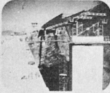
Boya de Montreuil (twin bridge) 5 spans: 47 + 3,160 + 47 = 274 m steel weight: 700 t precast concrete slab: 7,000 m 3
