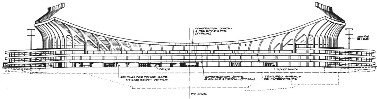
NORTHWEST ELEVATION
