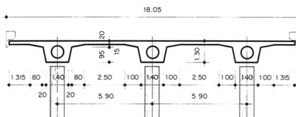
Fig. 1 Cross-section of the wadi crossing
