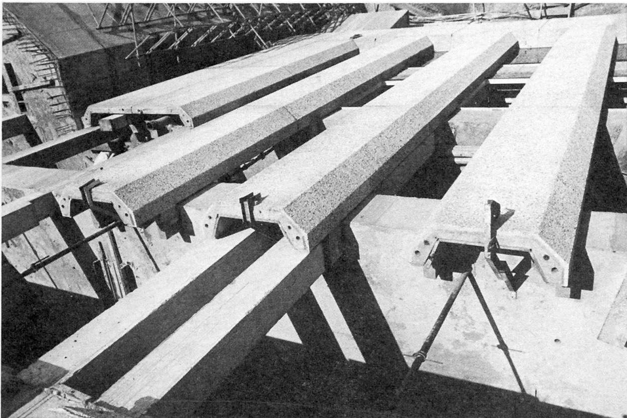
Fig. 4. Insulated precast concrete return air ducts being fixed to edge of structure
