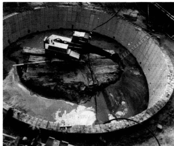
Excavation during sinking of the concrete basin, Ø 17 m; 16 m below the ground surface
