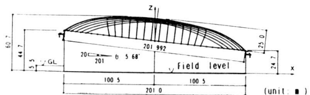
Roof structure outline
