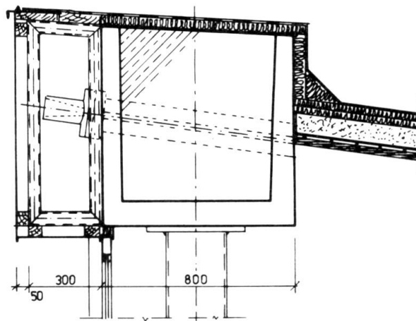
Fig. 5 Detail of the edge beam: Roofing-coat composition: Cable netting + F30 fire protection, welded wire-netting, glass texture, thermal insulation with glass-wool 100 mm, wood cement plates: 2×25 mm, water insulation with rubber foil, reflex paint.
