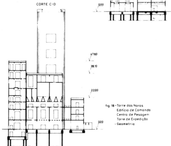
Fig. 3: Intake tower, control building, weighing center and outloading – Geometry
