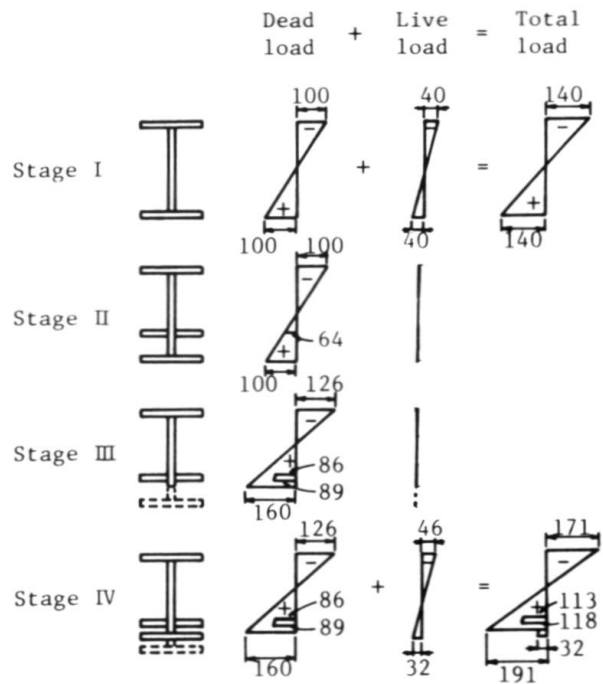
(K. Horikawa, H. Suzuki) Fig. 3 Schematic example of stress (MPa)
