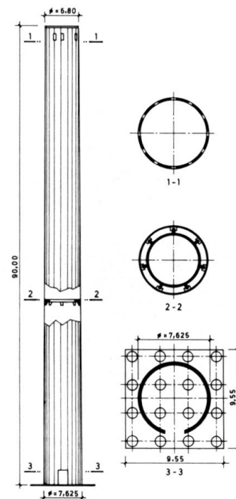
Fig. 2 Geometry of the chimney
