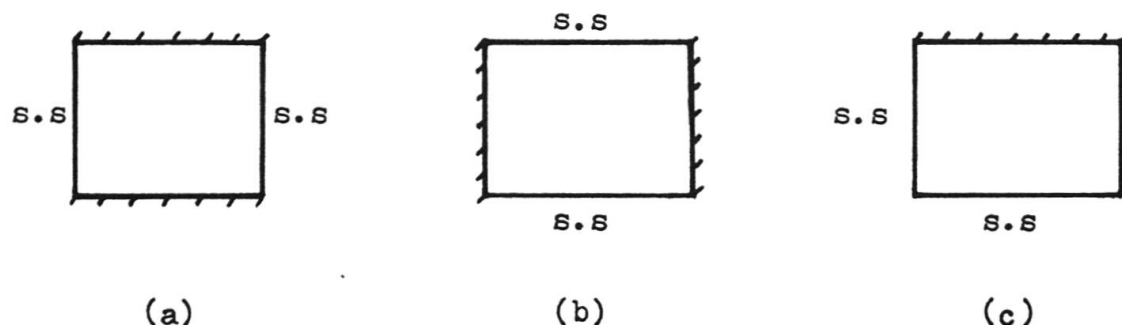
Fig. 4 Plates with 2 edges simple supported and 2 edges clamped
