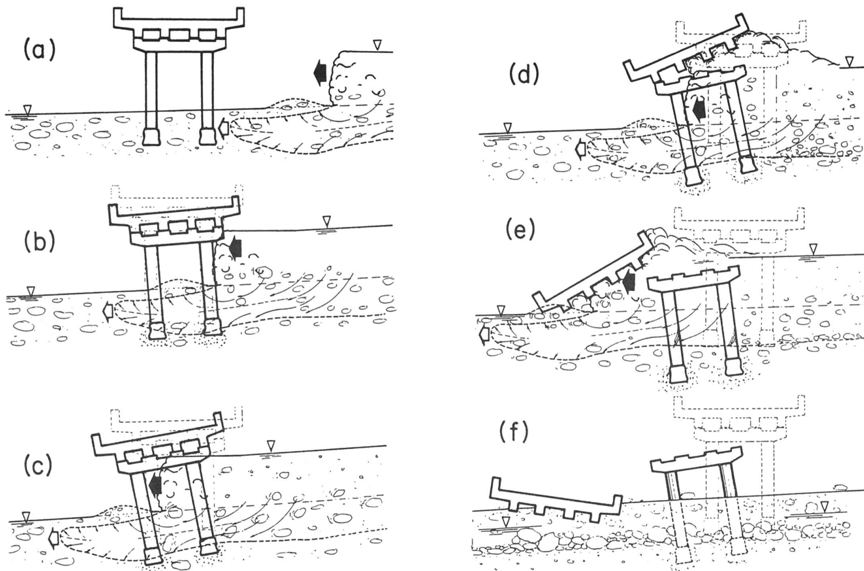
FIG. 4 SCHEMATICAL VIEW OF PROPOSED FAILURE MECHANISM
