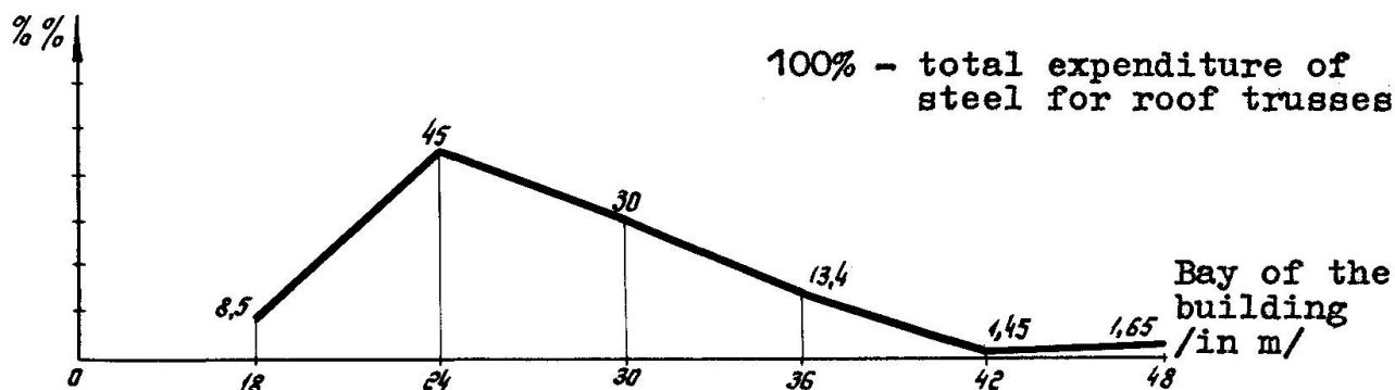
Fig. 1. Use of roof trusses in per cent in terms of the building bay
