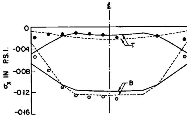
Figure 25 - Longitudinal Stresses Along Transverse Grid Line 4 All Cables Prestressed
