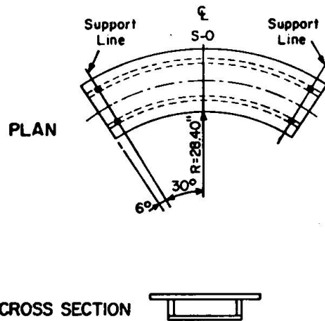
Figure 10 - Geometry of Box Girder Model
