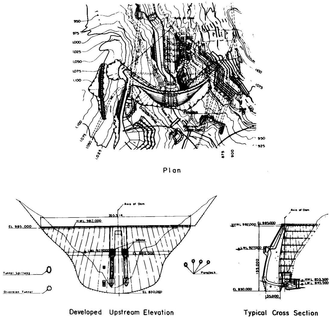
Fig.1 Features of Nagawado Dam
