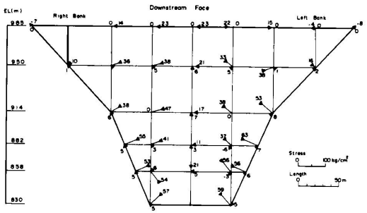
Fig.5 Principal Stress by F.E.M. (Static Load)
