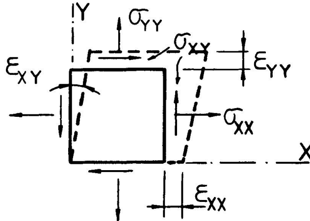
Fig. 2 Plane Element
